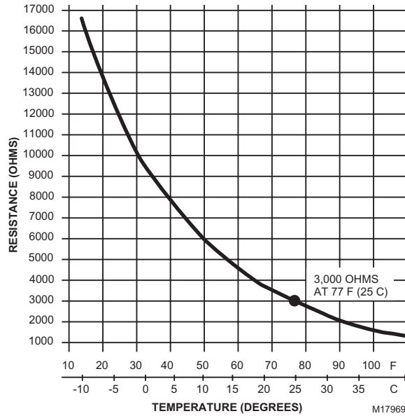
Fig. 3. C7150B1004 Sensor resistance temperature.
